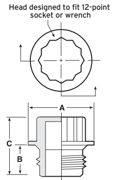
Caplugs No. P-48C
