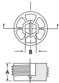
Caplugs No. P-68VH
