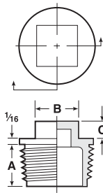
Caplugs Nos. P-68H and P-88H
